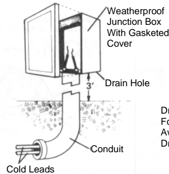
FIG. 1-D OUTDOOR ABOVE GRADE JUNCTION BOX MOUNTING
