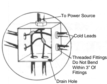
FIG. 1-C INDOOR PREFERRED JUNCTION BOX LOCATION
