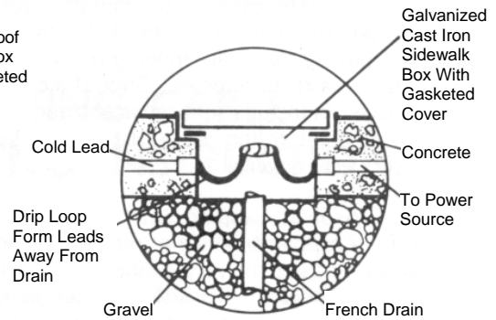
FIG. 1-E SIDEWALK JUNCTION BOX ARRANGEMENT AT GRADE LEVEL
